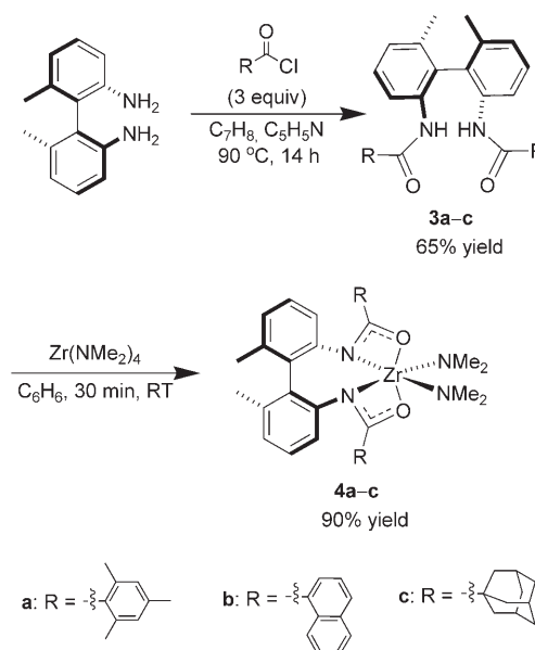
Scheme 1. Facile preparation of chiral Zr bis(amidate) complexes.
